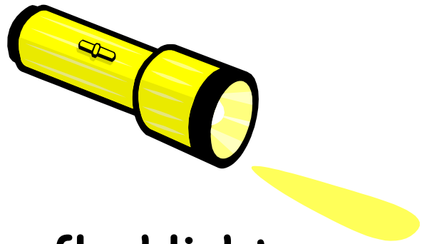
flashlight
