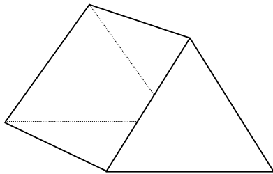
prism
