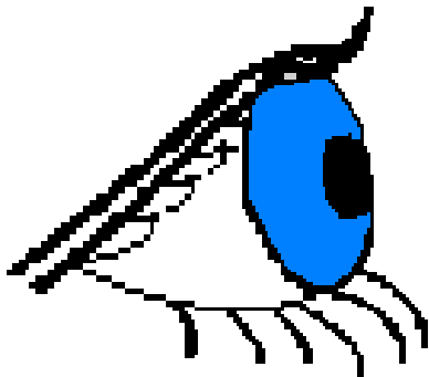
eye
