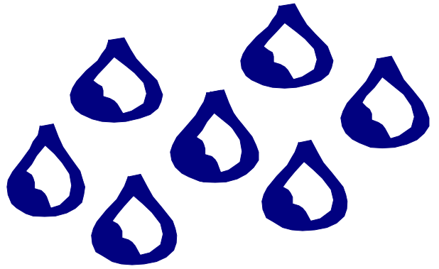
water drops
