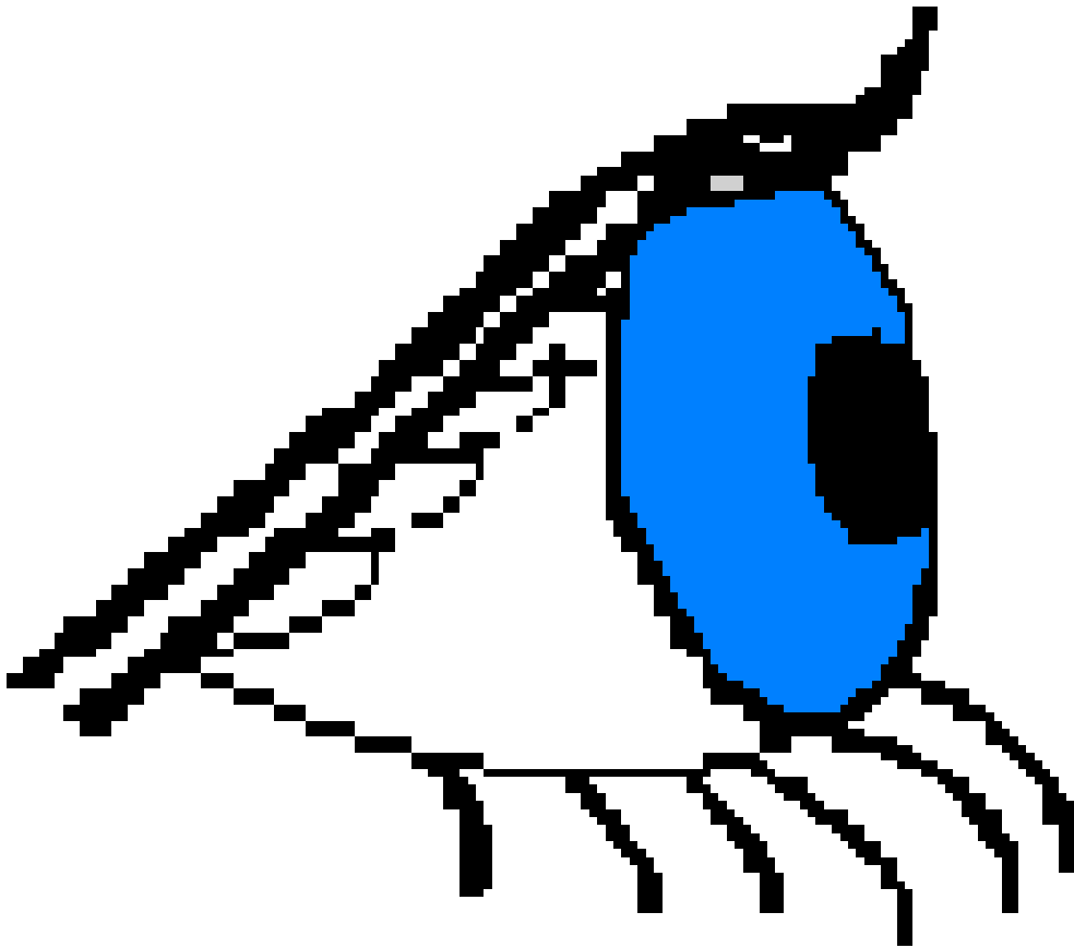
eye
